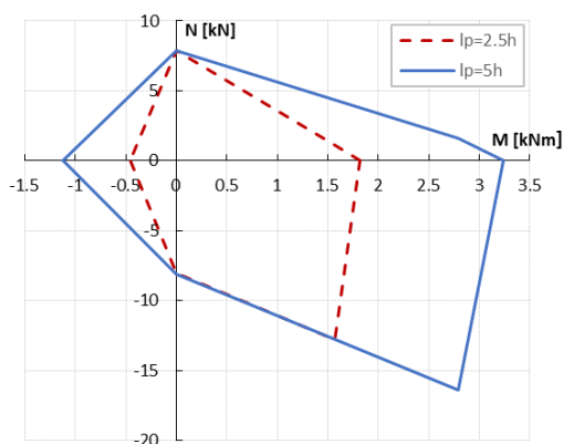
4K, 140/160, \alpha = 60^\circ
