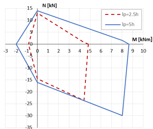
3K, 180/220, \alpha = 60^\circ
