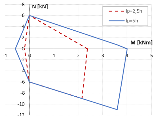
3K, 140/160, \alpha = 45^\circ
