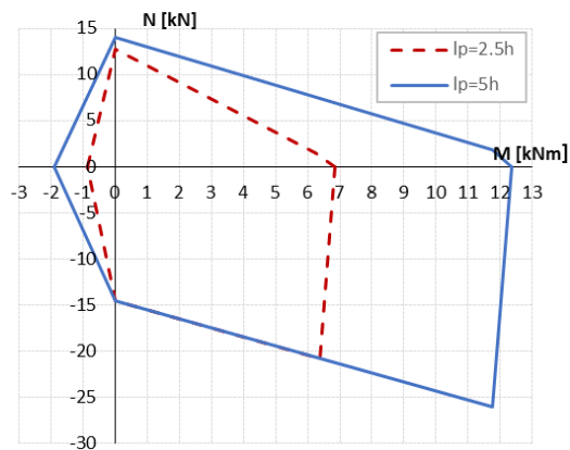
3K, 180/220, \alpha = 45^\circ
