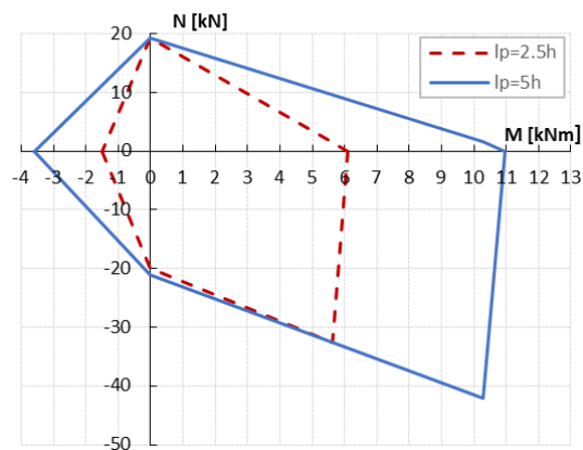
4K, 180/220, \alpha = 60^\circ
